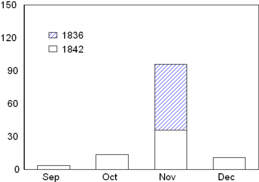
Figure 2. Off-reservation tribal deer harvest by month in Michigan ceded territories, 2004.
